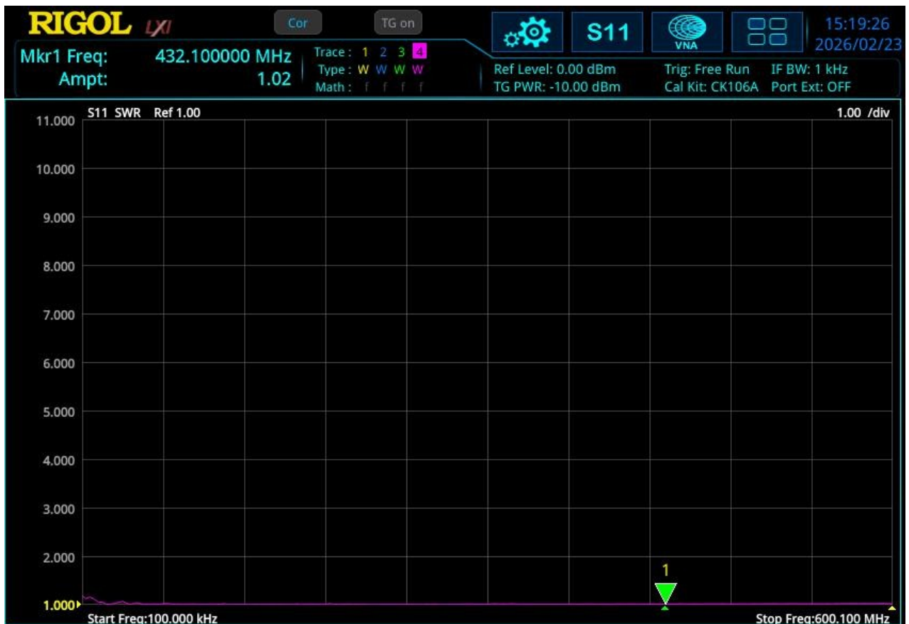
Figure 5: Standing Wave Ratio (SWR) vs Frequency
