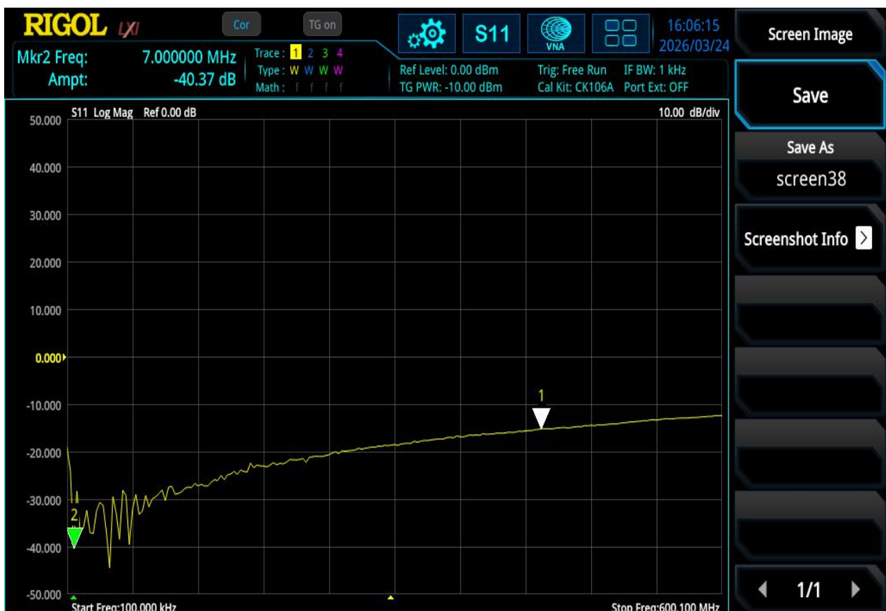
Figure 6: Return Loss vs Frequency
